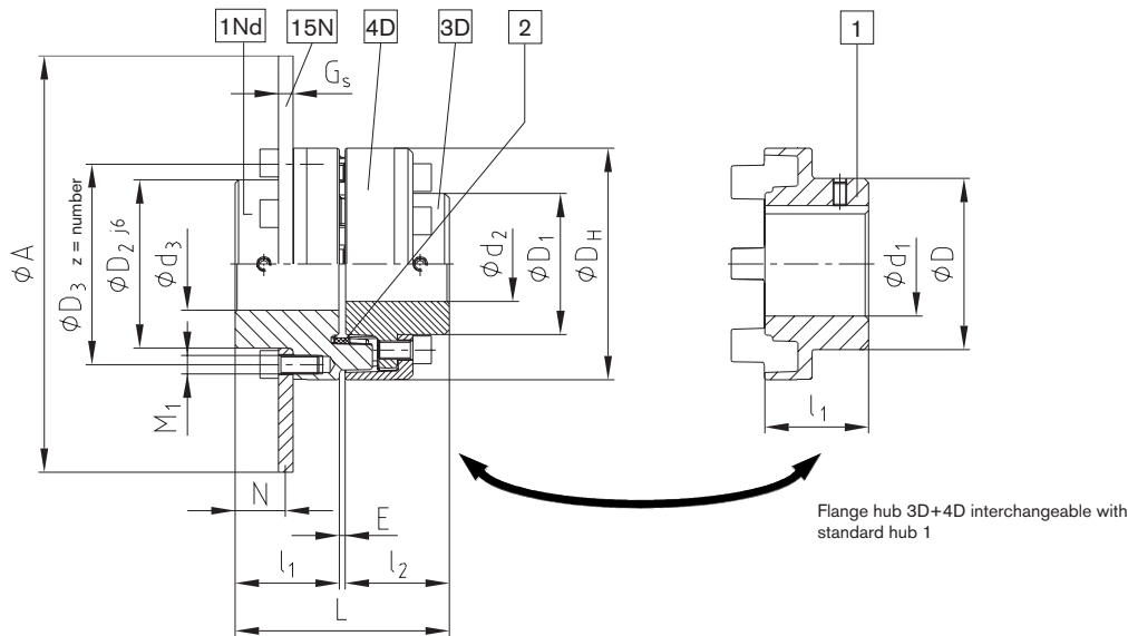
With standard hub type AR-BTA or AR-SBA
