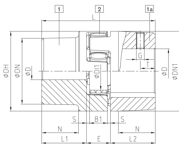
AI-D (thread opposite the keyway)
