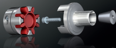
ROTEX® GS expansion hub
