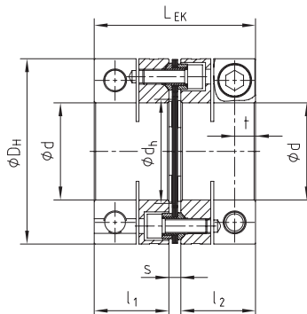
RADEX®-NC Types DK and EK - Hub and spacer material aluminium up to size 61, steel with size 75 / laminae made of stainless steel
