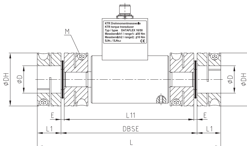
Dimensions [mm] of torque measuring shaft and coupling combination with RADEX®-NC HT
