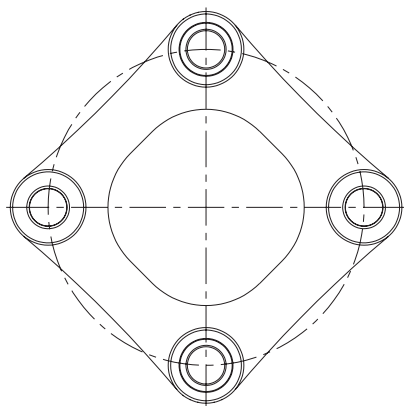
Size 5 to 26 (laminae with 4 holes)
