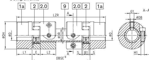
Type ZR (with GS spider)
