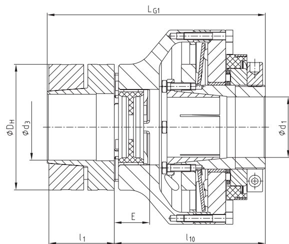
Hub type 6.0
