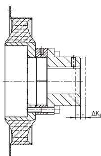
Axial displacement
