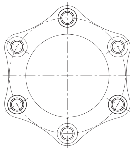
Size 36 to 75 (laminae with 6 holes)
